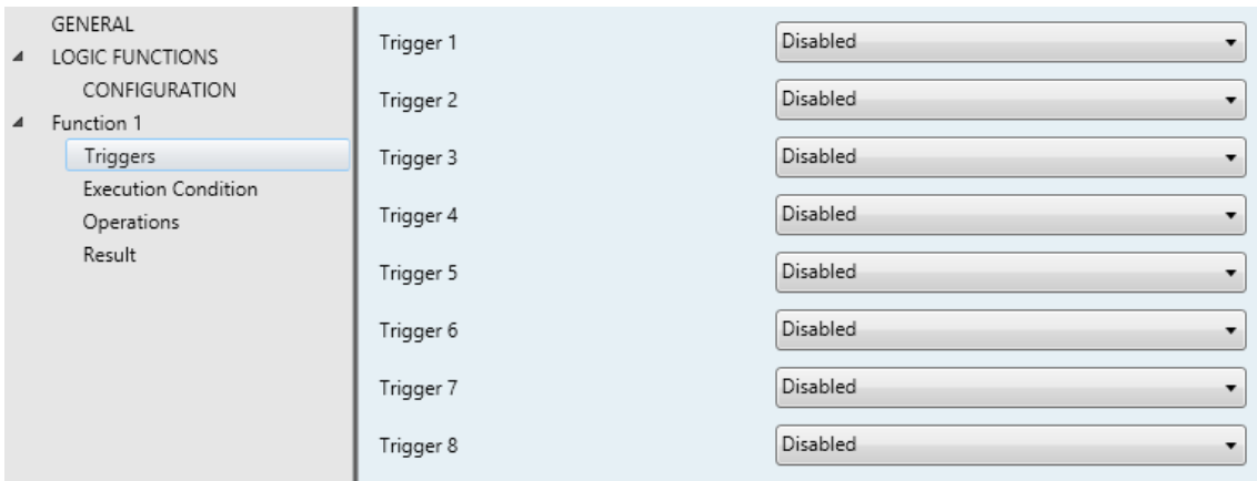
Figure 4. "Triggers" Tab
