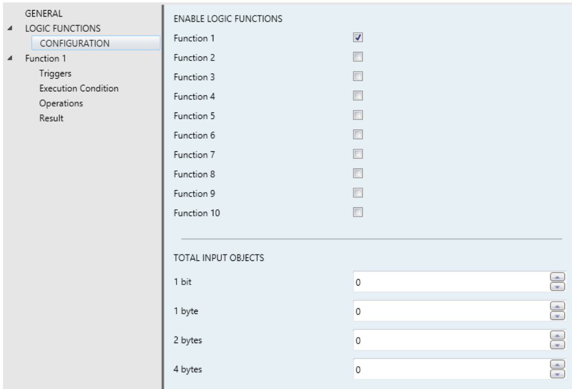
Figure 3. Function 1 enabled.
